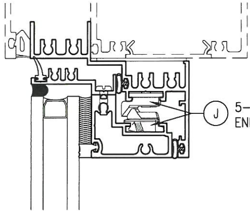
6 INTERLOCKING SNUBBER HEAD Scale: 6" = 1'-0"
