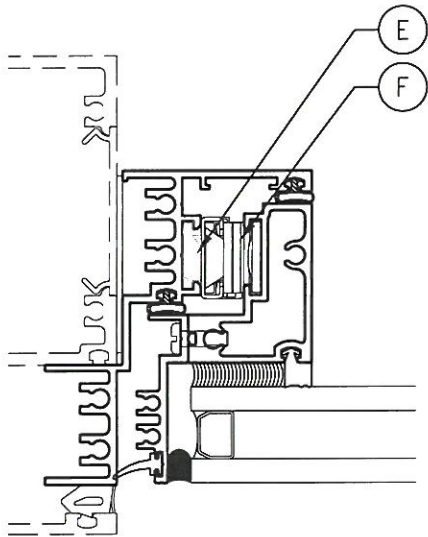
4 MULTI-POINT LOCK — HARDWARE JAMB/SILL Scale: 6" = 1'-0"
