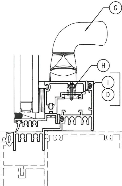
7 BI-DIRECTIONAL OPERATOR SILL Scale: 6" = 1'-0"
