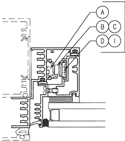
4 MULTI-POINT LOCK — HARDWARE JAMB/SILL Scale: 6" = 1'-0"
